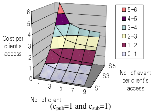
Fig. 2. Cost per client's access of publish/subscribe model ( c_{pub}=1 and c_{sub}=1 )
