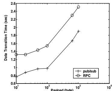
Fig. 4. Latency by Payload
