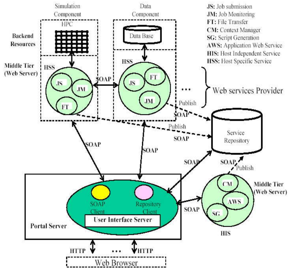
Fig. 1. Architecture of Web service-based computing portals.
